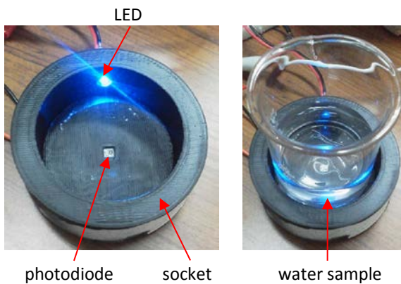
Fig. 2. Photograph of our optical measurement setup.
